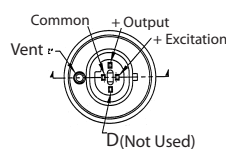
Top View: 4-Pin Packard Connector Type: Metri-Pack 150
