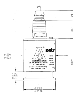
1 1/2" Tri-Clover Sanitary Fitting Diaphragm Material: 316SS
