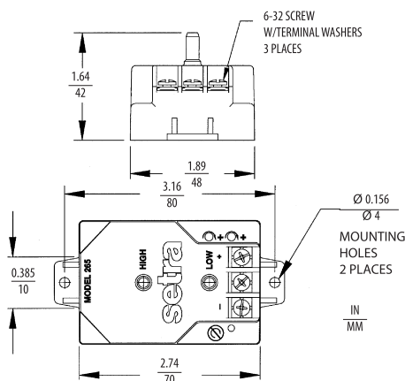
Code T1 Electrical Termination Dimensions
