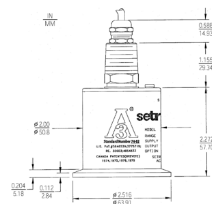
2" Tri-Clover Sanitary Fitting Diaphragm Material: 316LSS
